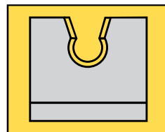
CN-12129 L= 23.5 mm H= 21 mm Ø 5 mm
