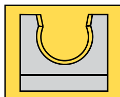
CN-12128 L= 23.5 mm H= 21 mm Ø 13 mm
