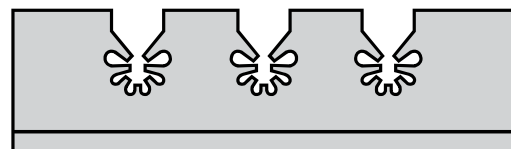
CN-12132 L= 72 mm H= 30 mm Instruments holder from Ø 3 to Ø 8 mm
